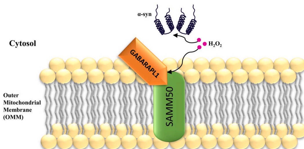
Fig. 5. Proposed interaction between molecules H_2O_2 and proteins ( \alpha -synuclein, GABARAPL1 and SAMM50) based on protein-protein interaction networks.
