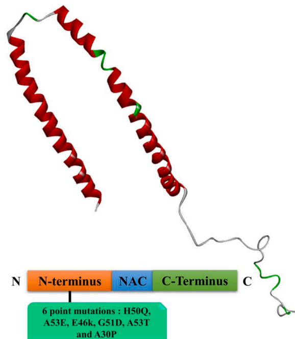
Fig. 2. \alpha -Synuclein and six point mutations.
