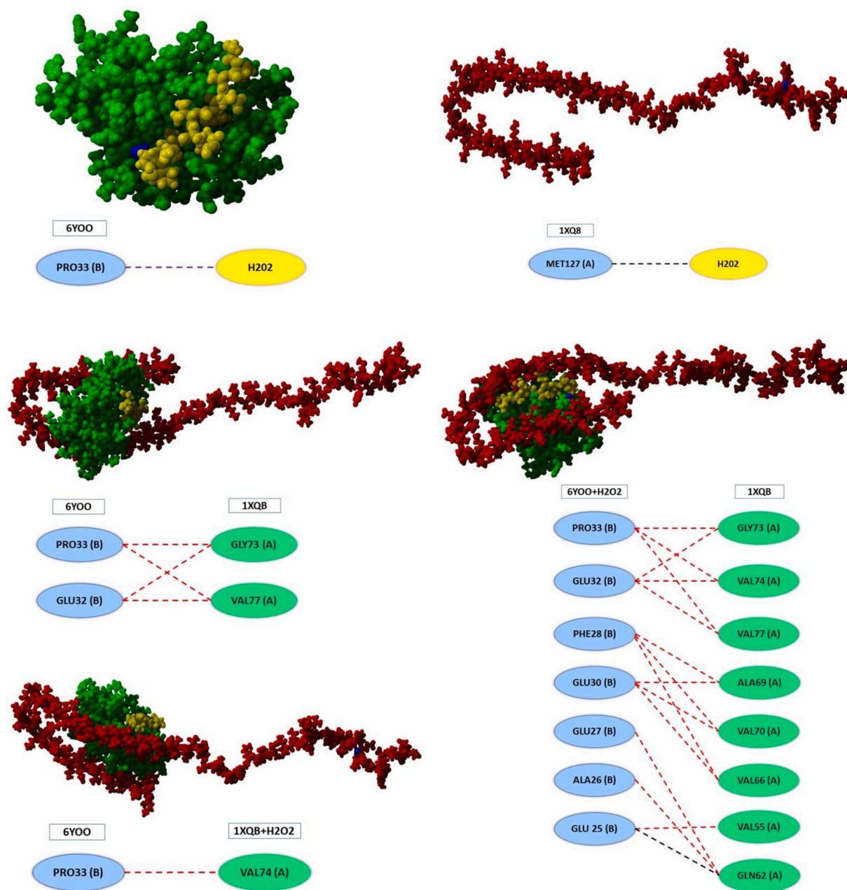
Fig. 7. Interaction between 1XQB ( \alpha -synuclein protein), 6YOO (GABARAPL1+SAMM50) and \text{H}_2\text{O}_2 . Colours description: 6YOO (Green: GABARAPL1; Yellow: SAMM50; Blue: \text{H}_2\text{O}_2 ), 1XQB (Red: \alpha -synuclein; Blue: \text{H}_2\text{O}_2 ) and Arrows (Red lines: Hydrophobic Bond; Black line: Hydrogen Bond). (For interpretation of the references to colour in this figure legend, the reader is referred to the Web version of this article.)
