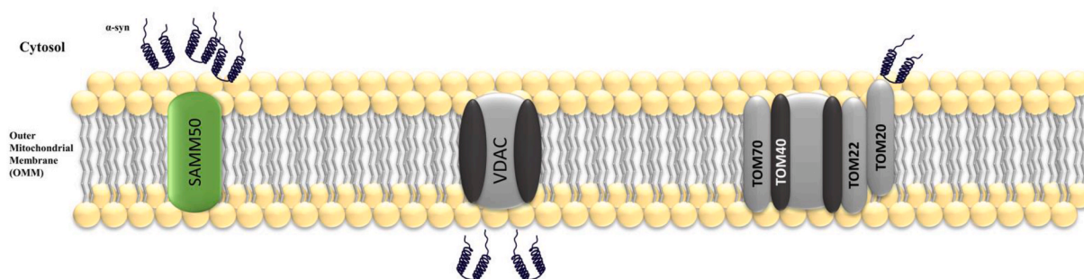
Fig. 1. Outer mitochondrial membrane and \alpha -synuclein.
