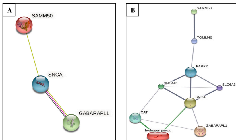
Fig. 4. Overview schematic of H_2O_2 addition to GABARAPL1+SAMM50 and \alpha -synuclein with (A) STRING and (B) STITCH database.
