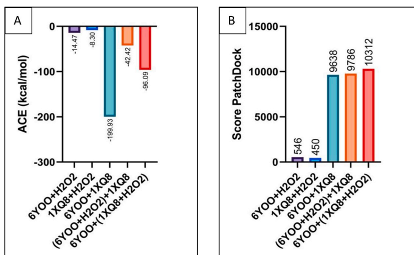
Fig. 6. PATCHDOCK score (A) ACE (Atomic Contact Energy) and (B) Docking score.
