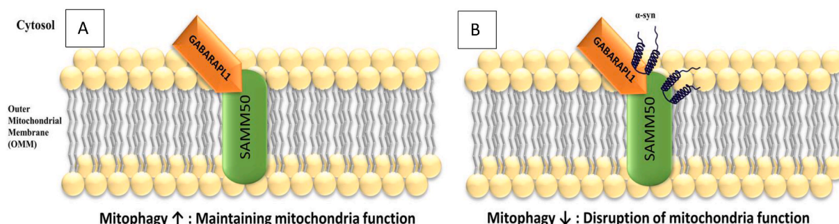
Fig. 3. Schematic model of SAMM50, GABARAPL1 and \alpha -synuclein association (A) Maintaining mitochondria function (B) Disruption of mitochondria function.
